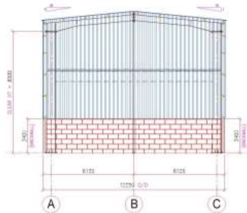
END WALL ELEVATION @ GL. 7
