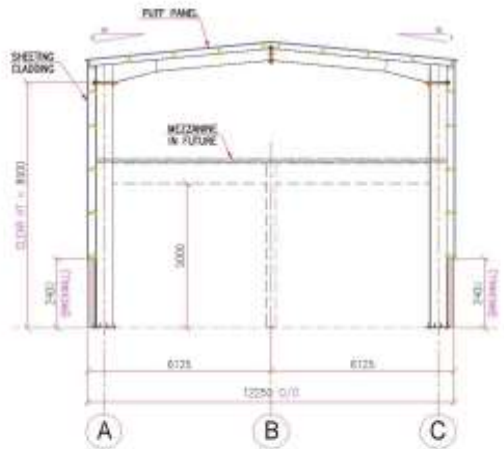
MAIN FRAME @ GL. 6
