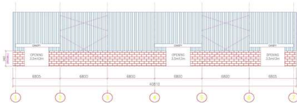
SIDE WALL ELEVATION @ GL. A
