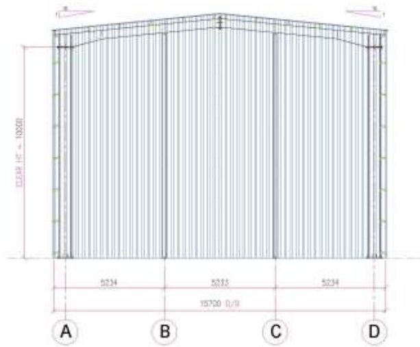
END WALL ELEVATION @ GL. 4
