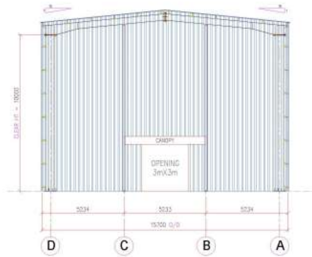
END WALL ELEVATION @ GL. 1
